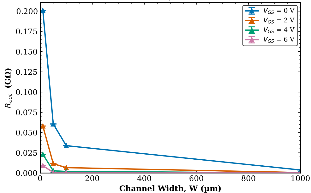
TFT1 Transistor 2 R_{out} vs W | L = 8\text{ }\mu\text{m}
